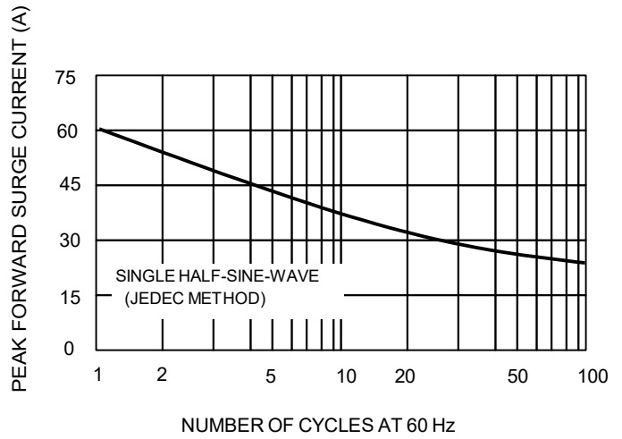
FIG.2: Forward Surge Current Capability
